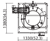
Dimensions [mm(in)]
